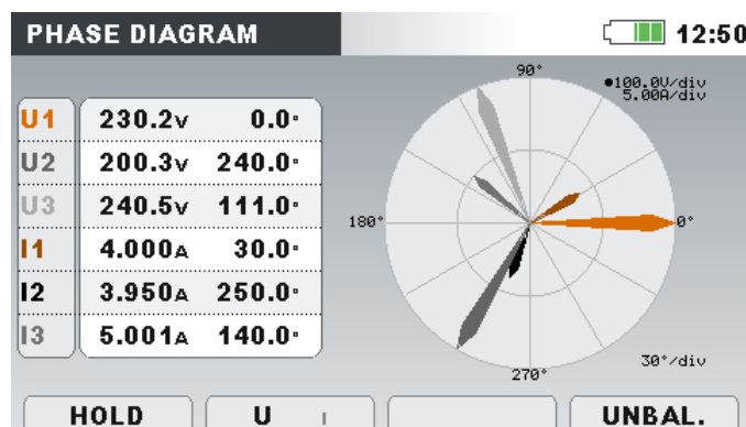
Image0.36: Ecran diagramme de phase
