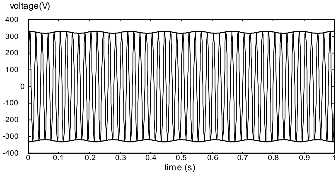
Image 0.8: Fluctuation de tension
